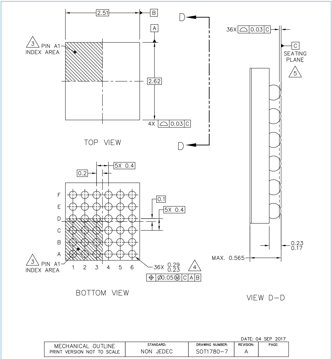
Figure 13-2: Package outline WLCSP36 (SOT1780-7); with back side coating
