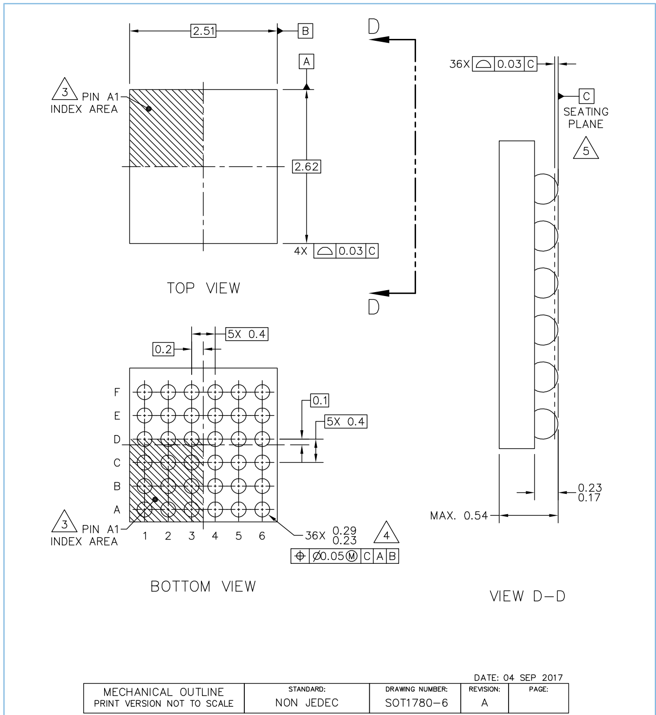
Figure 13-1: Package outline WLCSP36 (SOT1780-6); no back side coating
